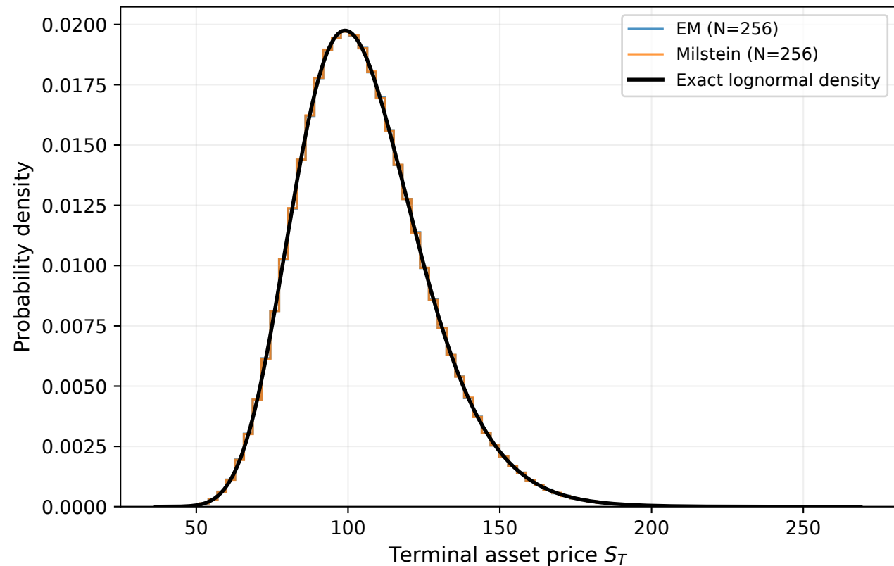
GBM terminal distribution; M=2,000,000; seed=32104
